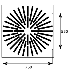
Difuzor BD9-KR-800
